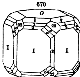
St. Gothard.
